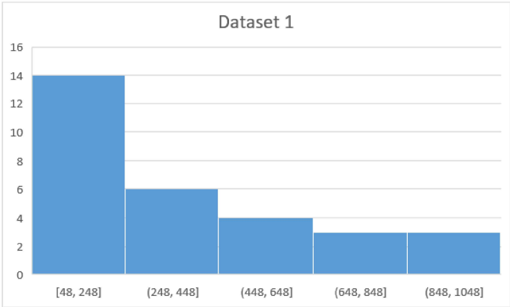
Strong positive skewness (right skew)
