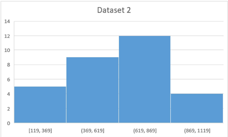
Weak negative skewness (left skew)
